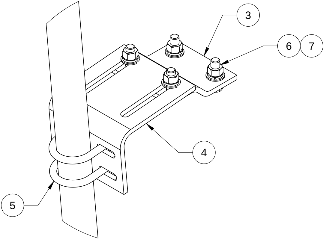
DETAIL A
